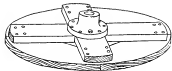
FIG. 548. WOOD FACE-PLATE FOR LARGE WORK.
